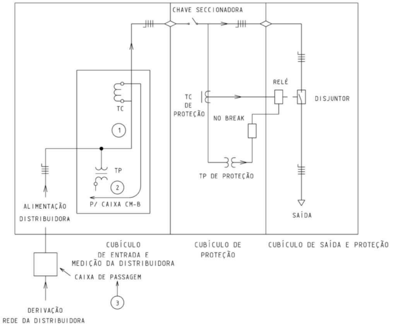
DIAGRAMA UNIFILAR
