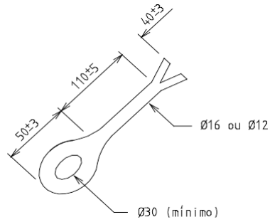
CHUMBADOR – OLHAL
